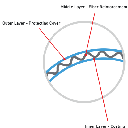
The NORDILONG has a three-layered structure design
